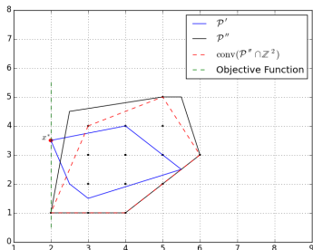
(a) Original LP relaxation
