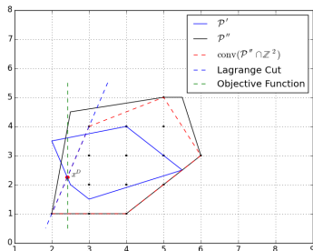
(b) After adding Lagrange cut
