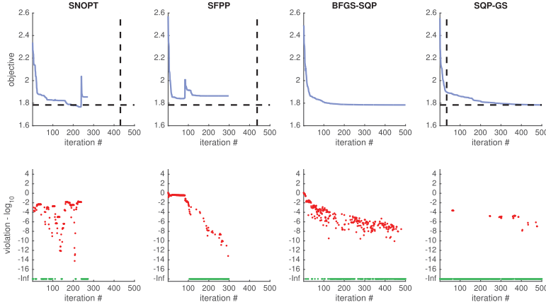
Figure A7. The plots in the top row track the value of the pseudospectral-radius-based objective function in terms of iteration number for SNOPT, SFPP, BFGS-SQP, and SQP-GS (left to right) on a randomly generated example of dimension N = 7 comprised of two plants in the objective and three in the constraint and where the controller matrix has MP = 5 \times 4 = 20 variables. In the top row of plots, the vertical dashed line indicates the iteration number whose elapsed CPU-time was closest to BFGS-SQP total elapsed CPU-time while the horizontal dashed line indicates the value of BFGS-SQP's best feasible solution. The log 10 -scaled plots in the bottom row show the amount of violation tracking with the iteration counts with '-Inf' indicating zero violation (feasible points).
