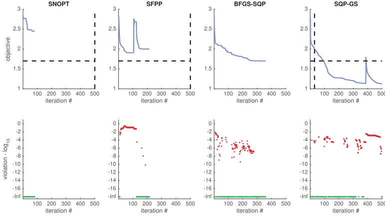
Figure A3. The plots in the top row track the value of the spectral-radius-based objective function in terms of iteration number for SNOPT, SFPP, BFGS-SQP, and SQP-GS (left to right) on a randomly generated example of dimension N = 10 comprised of one plant in the objective and four in the constraint and where the controller matrix has MP = 16 \times 1 = 16 variables. In the top row of plots, the vertical dashed line indicates the iteration number whose elapsed CPU-time was closest to BFGS-SQP total elapsed CPU-time while the horizontal dashed line indicates the value of BFGS-SQP's best feasible solution. The \log_{10} -scaled plots in the bottom row show the amount of violation tracking with the iteration counts with '-Inf' indicating zero violation (feasible points).
