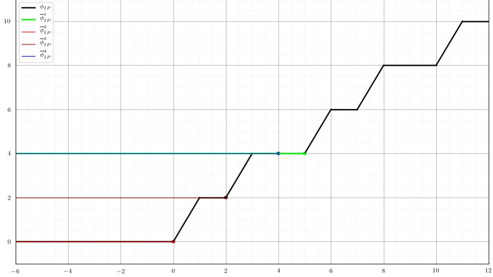
Figure 7: Primal functions constructed in the algorithm for solving (38)
