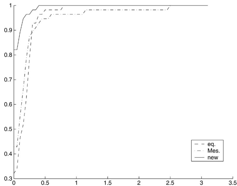
Fig. 3. Performance profile for iteration counts.
